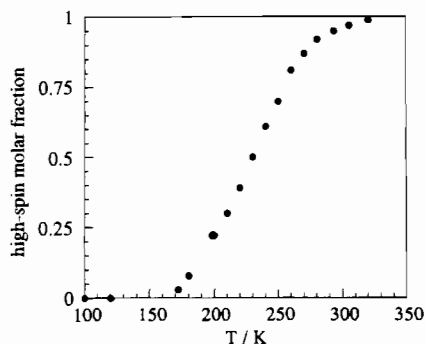
Figure 6. High-spin molar fraction versus temperature for the central iron(II) ion of compound 2a \cdot 4H_2O as deduced from the Mössbauer spectra.
