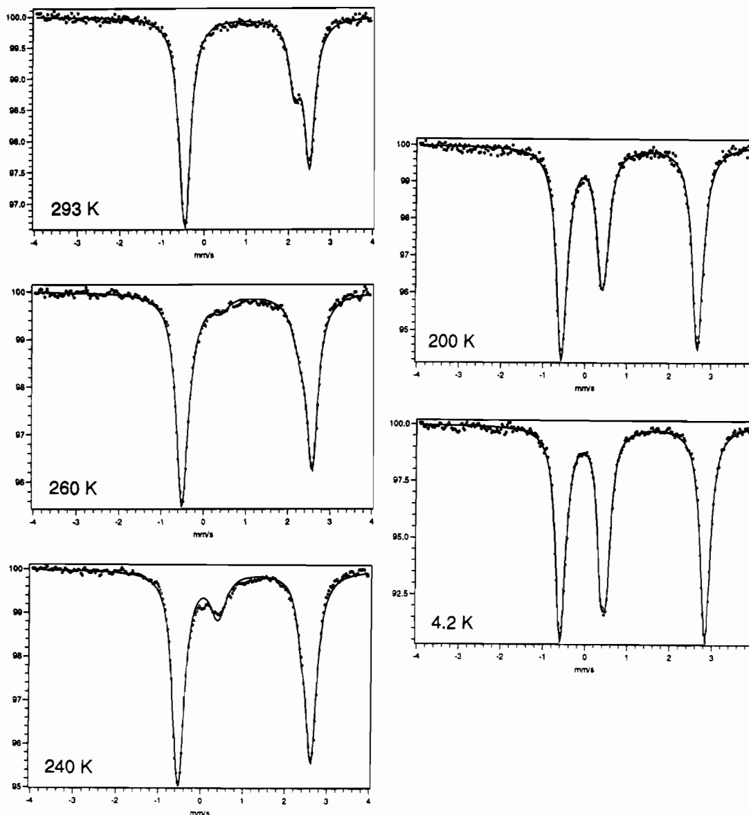
Figure 5. Mössbauer spectra of compound 2a \cdot 4H_2O at various temperatures.
