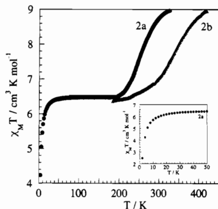
Figure 4. \chi_M T versus T plots for compounds 2a · 4\text{H}_2\text{O} and 2b . The insert emphasizes the data below 50 K for 2a .
