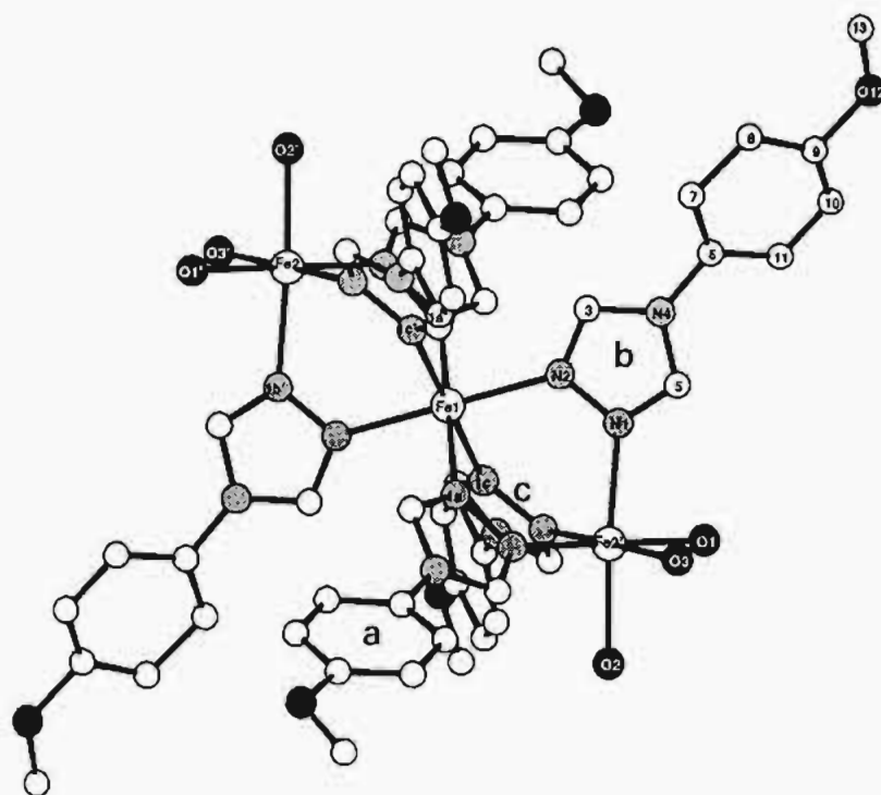
Figure 2. View of the [\text{Fe}_3(\text{p-MeOptrz})_6(\text{H}_2\text{O})_6]^{6+} trinuclear cation in compound 2\text{a} \cdot 2\text{CH}_3\text{OH} \cdot 8\text{H}_2\text{O} . H-atoms were omitted for clarity. Oxygen atoms are black, and nitrogen atoms are shaded.
