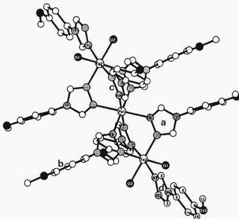
Figure 1. View of the [\text{Fe}_3(\text{p-MeOptrz})_6(\text{H}_2\text{O})_4]^{6+} trinuclear cation in compound 1 \cdot 2\text{H}_2\text{O} . H-atoms were omitted for clarity. Oxygen atoms are black, and nitrogen atoms are shaded.
